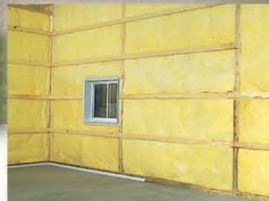
Super insulated building packages to meet or exceed energy standards. ● R19 to R25 Walls ● R40 to R50 Ceilings
